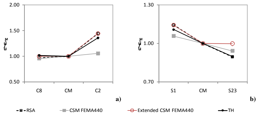
Fig. 8 – Normalized top displacements a) three storey building, X direction, 0.1g, b) five storey building, X direction, 0.1g.
