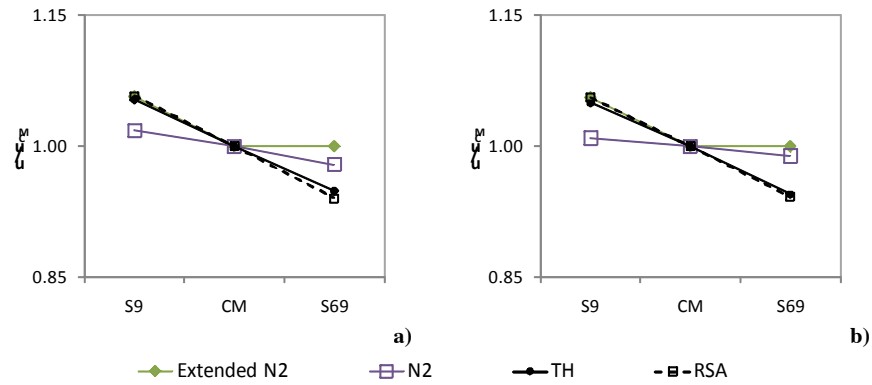
Fig. 7 – Normalized top displacements, eight storey building a) X direction, 0.2g, b) X direction, 0.4g.
