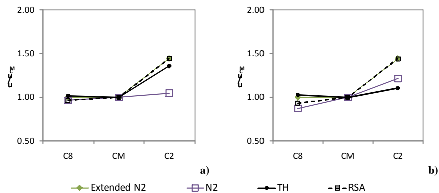
Fig. 5 – Normalized top displacements, three storey building a) X direction, 0.1g, b) Y direction, 0.2g.
