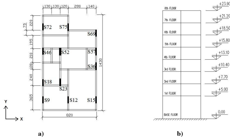
Fig. 3: Eight storey building configuration (a) Plan View (cm), (b) Lateral View (m).
