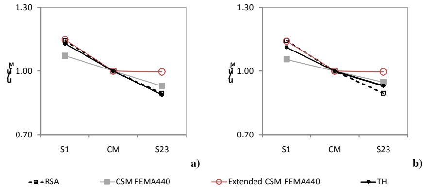
Fig. 9 – Normalized top displacements, five storey building a) X direction, 0.2g, b) X direction, 0.6g.
