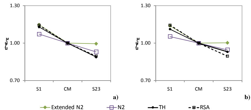
Fig. 6 – Normalized top displacements, five storey building a) X direction, 0.2g, b) X direction, 0.6g.
