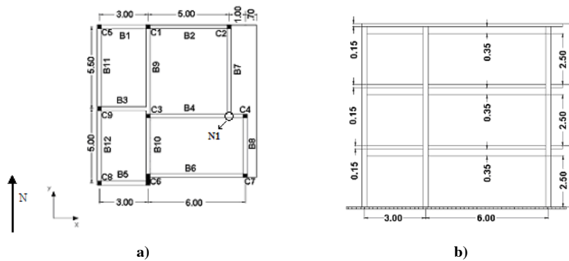
Fig. 1: Three storey building configuration: a) in plan; b) at the south west facade (units in meters).
