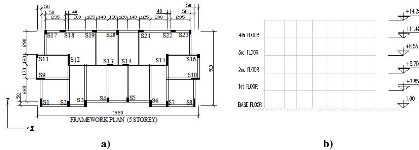
Fig. 2: Five storey building configuration (a) Plan View (cm), (b) Lateral View (m).
