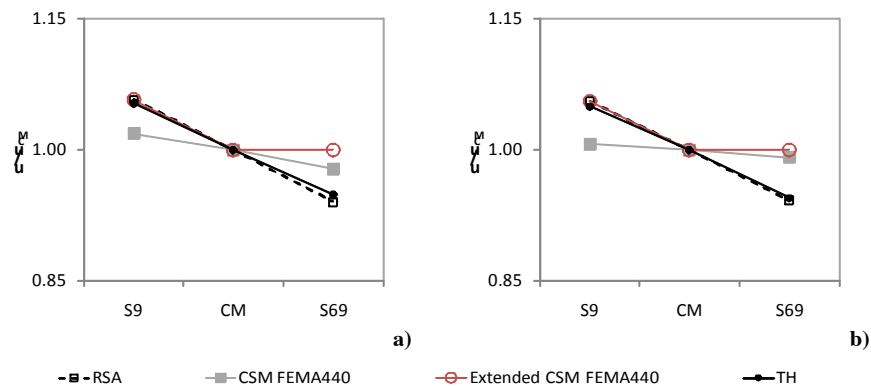
Fig. 10 – Normalized top displacements, eight storey building a) X direction, 0.2g, b) X direction, 0.4g.
