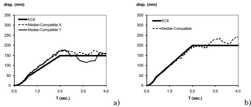
Fig. 4 – Displacement response spectra a) three storey, b) five and eight storey buildings.
