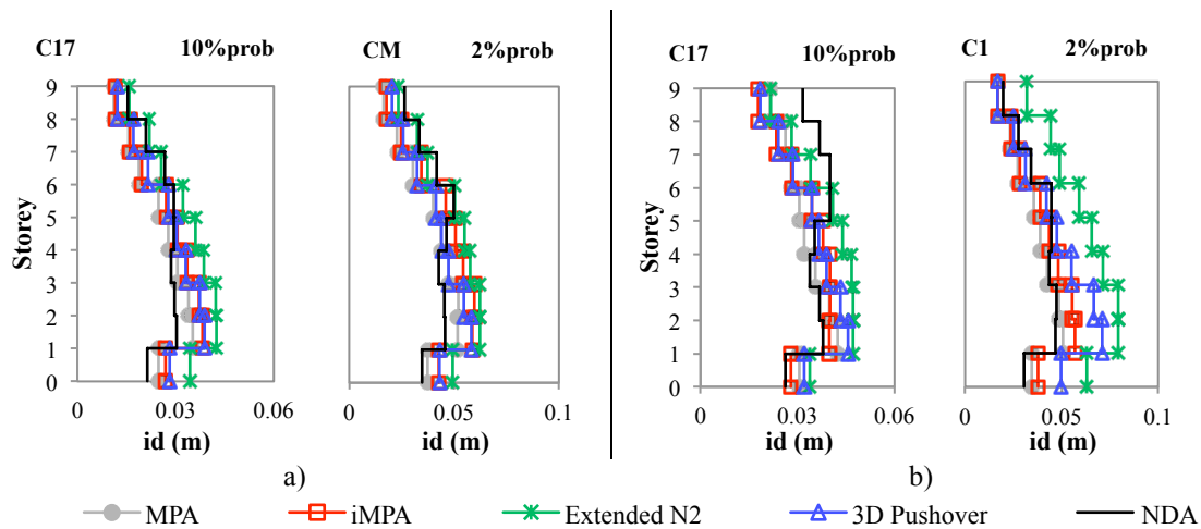
Figure 8 – Interstorey Drifts - a) X direction; b) Y direction
