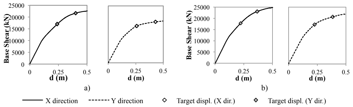
Figure 5 - Pushover curves in X and Y direction, respectively: a) Extended N2; b) 3D Pushover
