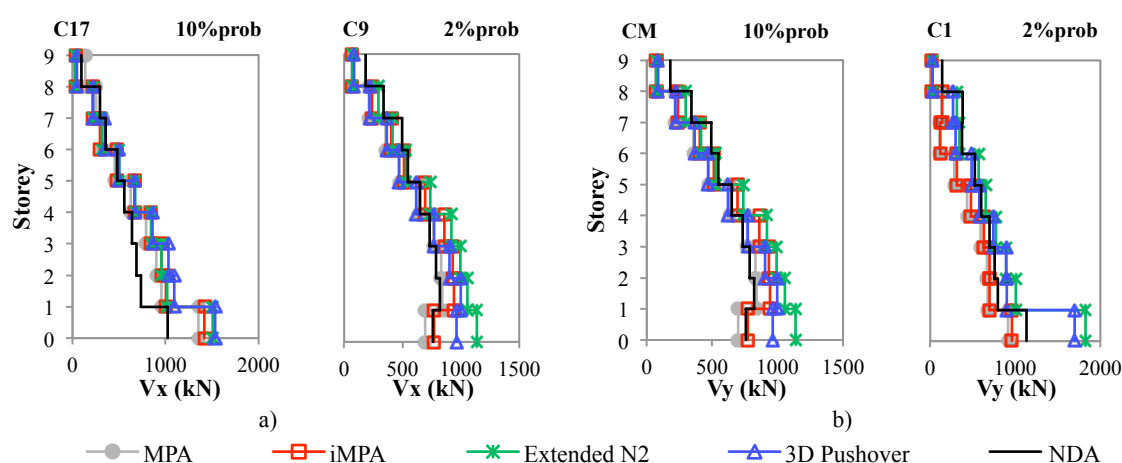
Figure 10 – Shear Forces: a) X direction; b) Y direction
