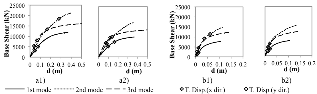
Figure 3 – Pushover curves of the 3 modes in MPA procedure: a1) 1 st triplet of modes, X direction; a2) 1 st triplet of modes, Y direction; b1) 2 nd triplet of modes, X direction; b2) 2 nd triplet of modes, Y direction
