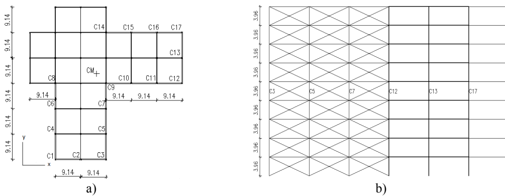
Figure 1 – Case Study; a) Plan view; b) Lateral View, dimensions in [m] (Belejo and Bento 2013)
