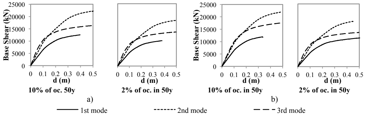
Figure 4 – Pushover curves of the 2 nd phase in iMPA procedure: a) X direction; b) Y direction
