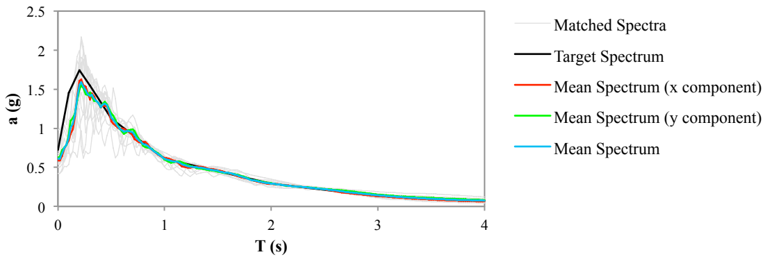
Figure 2 – Seismic Hazard Spectrum and the median response spectra of 7 scaled ground motions (x and Y directions and overall): a) SPEAR building; b) 9-Storey building
