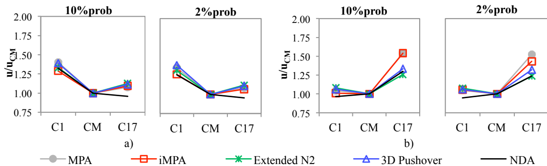
Figure 9 – Normalized Top displacements: a) X direction; b) Y direction
