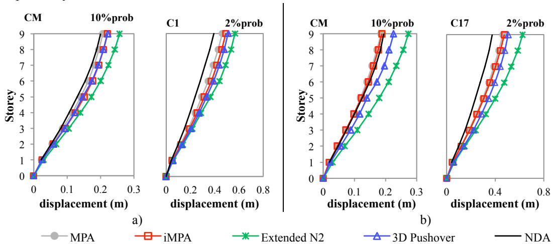
Figure 7 – Lateral Displacement Profiles: a) X direction; b) Y direction
