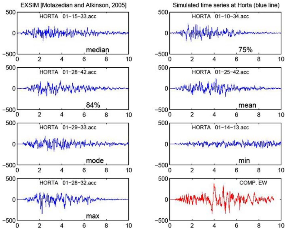
Fig. 7 Simulated time series. Simulated time series derived for the median, 75th (75%) and 84th (84%) percentiles, mean, mode, minimum and maximum PGA ( \text{cm}/\text{sec}^2 ). Each time series represents the one (among all of the 480 time series) that is closest to these absolute values. Red , recorded E–W component waveform at the Horta site
