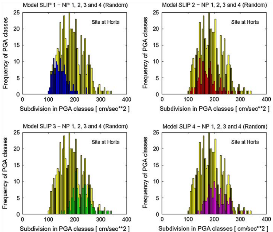
Fig. 8 Frequency of PGA classes versus PGA for the four slip models. Yellow bars , EPI 2; blue bars , SLIP 1; red bars , SLIP 2; green bars , SLIP 3; magenta bars , SLIP 4
