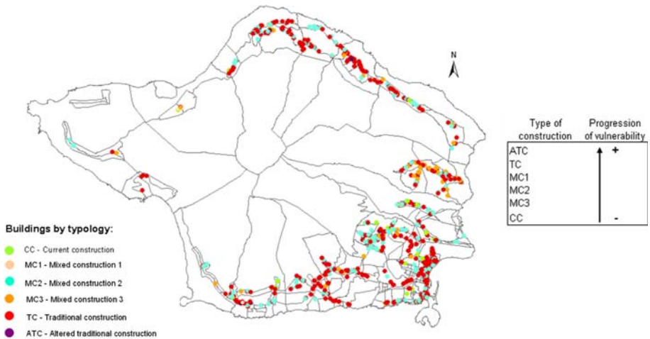
Fig. 11 Distribution of building types on Faial Island. Main panel: colour-coded spatial building distribution by construction class. Right panel: relationships between construction classes and vulnerability
