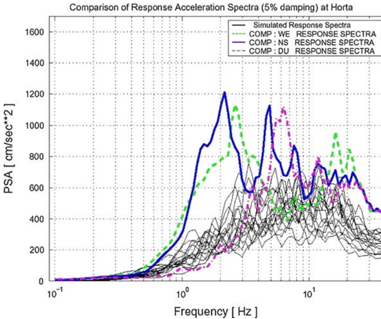
Fig. 9 Comparison of the response acceleration spectra at Horta. Acceleration spectra (5% damping) at Horta station for the horizontal components. Recorded responses: blue , NS; green , WE; magenta , DU. Simulated response: black
