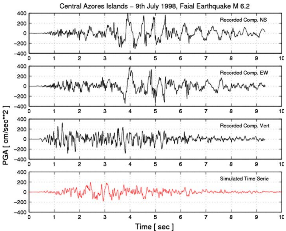
Fig. 3 Comparison between recorded and simulated records. Top three panels (black lines) : accelerometer time histories recorded at the Horta site (Faial Island). Bottom panel (red line) : horizontal component of an accelerogram computed using EXSIM (average of two). The simulation was carried out with EPI 2 (see Table 1), the model parameters are listed in Table 2, and the automatic random slip distribution was performed with nucleation point 2 (bilateral rupture)
