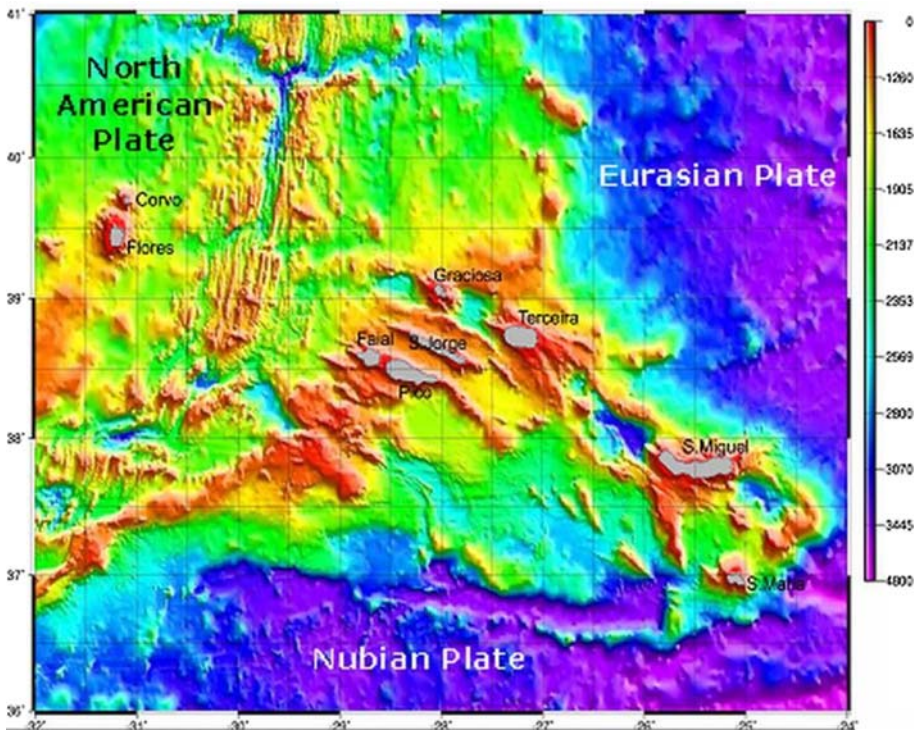
Fig. 1 Colour-coded bathymetry of the Azores plateau. Corvo and Flores Islands (western group); Graciosa, Terceira, Faial and Pico Islands (central group); São Miguel and Santa Maria Islands (eastern group). Redrawn after Lourenço et al. (1998)
