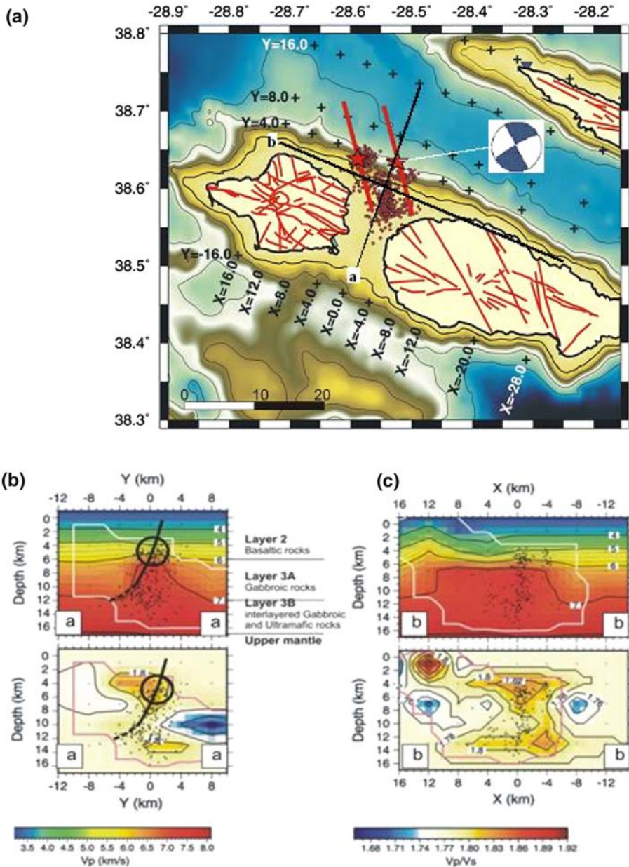
Fig. 2 Tectonic map of the central Azores Islands. a Simplified tectonic map of the central Azores Islands (Faial, left; Pico, right). Red lines, faults; red circles, epicentres of the seismic sequence triggered by the 1998 Faial earthquake; red stars, epicentre locations according to the EPI 1 and EPI 2 (see text) fault-plane solutions (after Senos et al. 2008); X, Y, location of the profiles for 3D tomography (Dias et al. 2007); b , c Tomographic cross-sections along the line from a to b on the map. Top panel, P-wave velocity colour-coded maps; bottom panel, V_p/V_s ratio colour-coded maps
