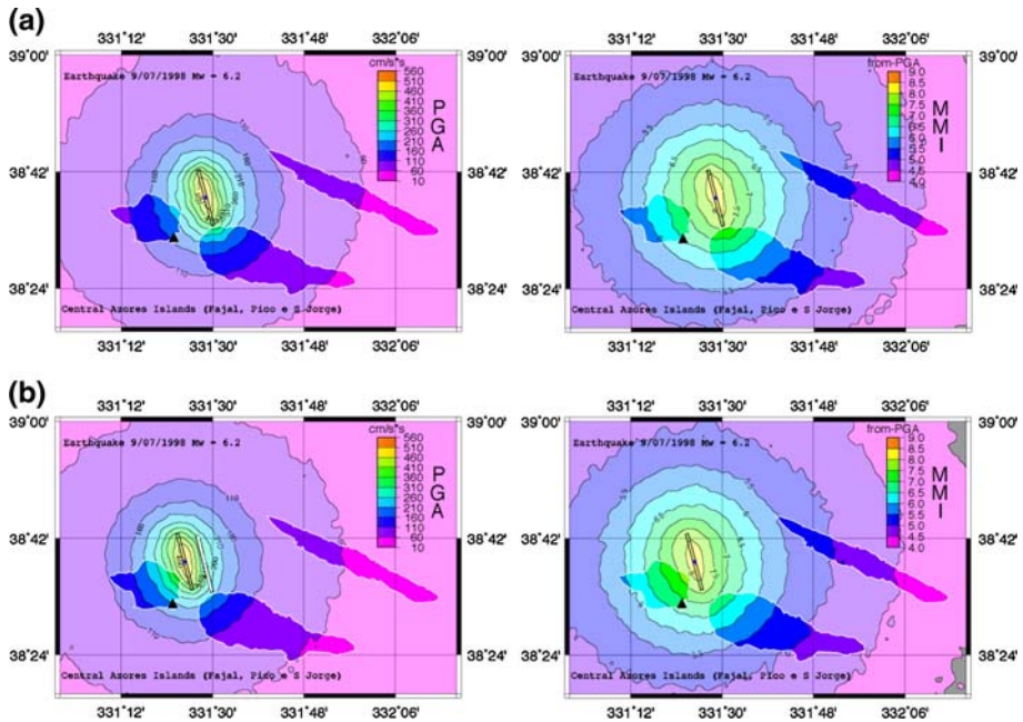
Fig. 5 PGA and MMI maps for the central Azores Islands (Faial, Pico and S. Jorge). The maps were computed on a 0.02^\circ \times 0.02^\circ grid using EXSIM, and the parameters are listed in Table 2. a Maps using EPI 1, and the location of EPI 1; b Maps using EPI 2, with the location of EPI 1 shown for comparison. Intensity was computed from the PGA ( \text{cm/s}^2 ) using Relationship (1) (Wald et al. 1999). Black triangle , the Horta site on Faial Island
