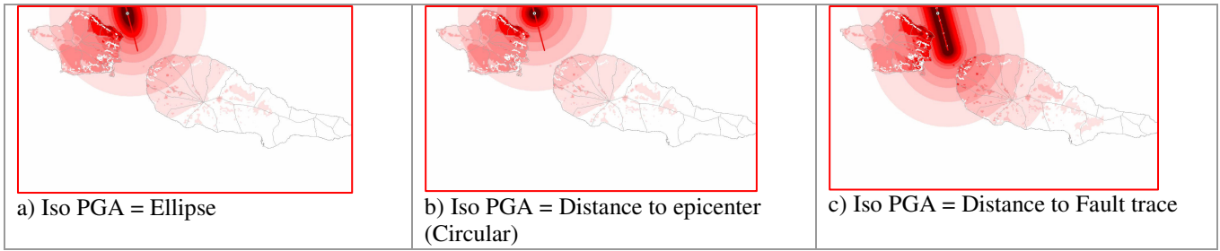
Figure 3 Propagation of seismic waves: different approaches
