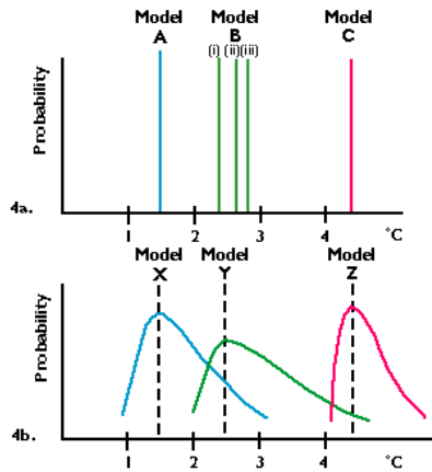
Figure 4. The Nature of GCM Results for 2 x CO 2 Climate Sensitivity
